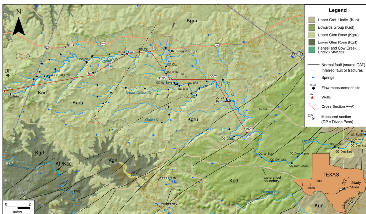
Figure 1. Location map of study area. Geologic base map from the Geologic Atlas of Texas (GAT). All sites are indicated (n = 69), but only the main channel of Onion Creek results (n = 22) are labeled and in Table 1.
