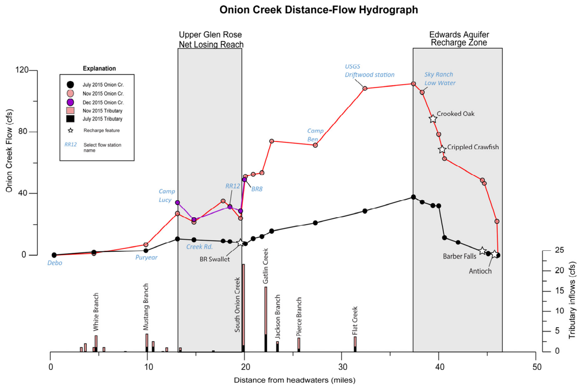
Figure 7. Flow in the main channel of Onion Creek plotted versus distance.
