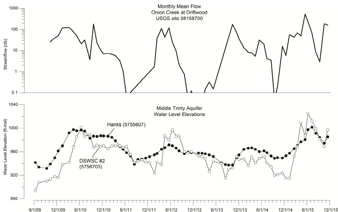
Figure 10. Hydrograph showing Onion Creek flows versus the Hanks well (5755607; TWDB, 2016a) and DSWSC #2 (5756703; HTGCD unpub. data), which are Middle Trinity Aquifer wells adjacent to Onion Creek. Note during wet periods, the DSWSC #2 well has a higher elevation than the upgradient Hanks well, which is located 3.8 miles to the northwest.
