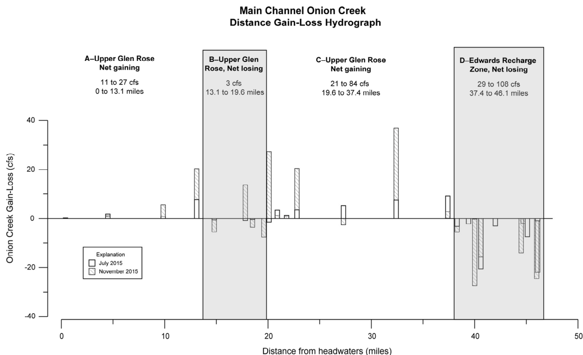
Figure 8. Flow gains and losses plotted versus distance. Data at each site represent the gain or loss from the preceding site immediately upstream in the main channel of Onion Creek.
